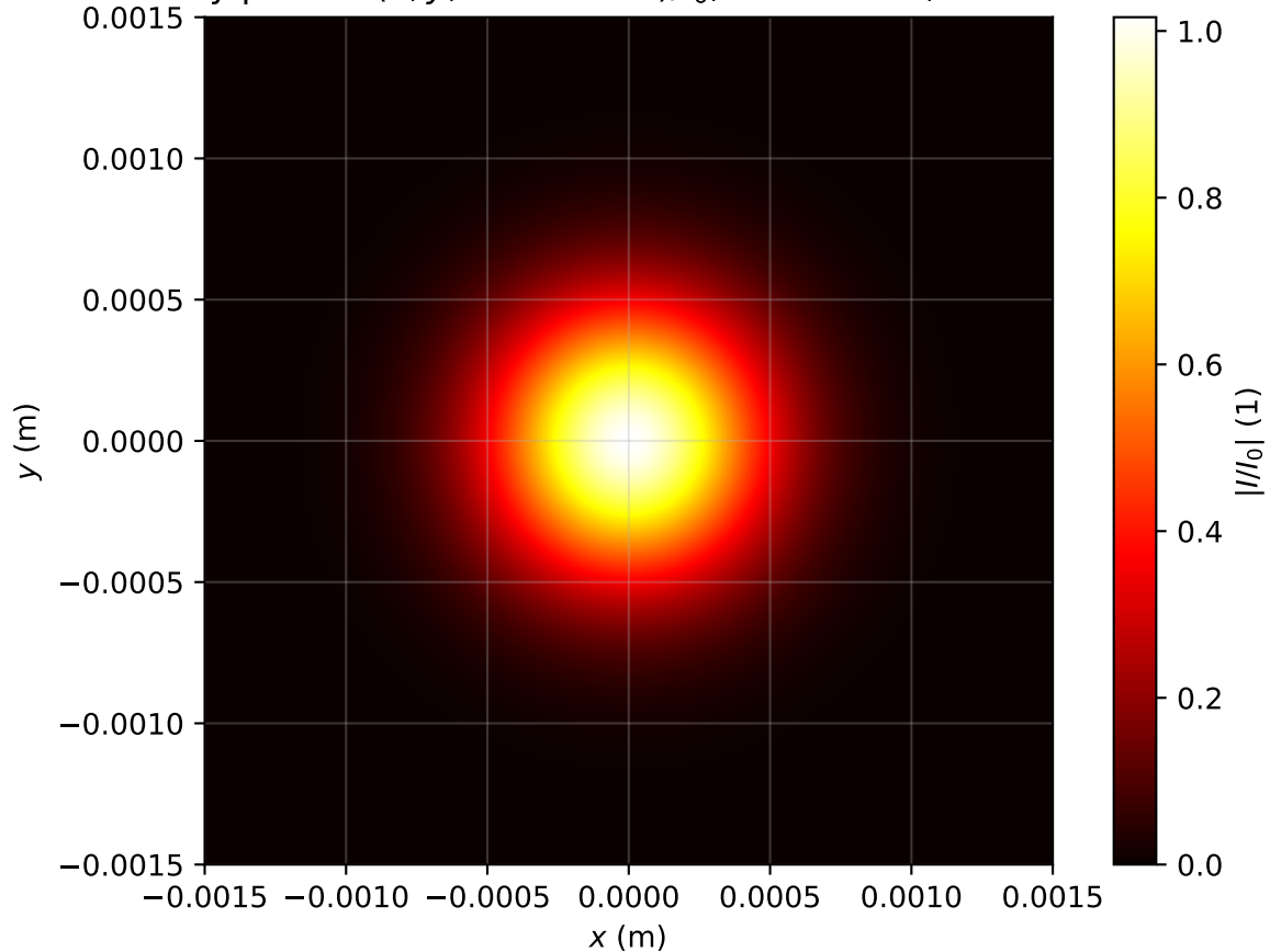
Intensity profile I(x, y, z = 0.159m)/I_0 , Pin=0.9Pcr, artificial time
